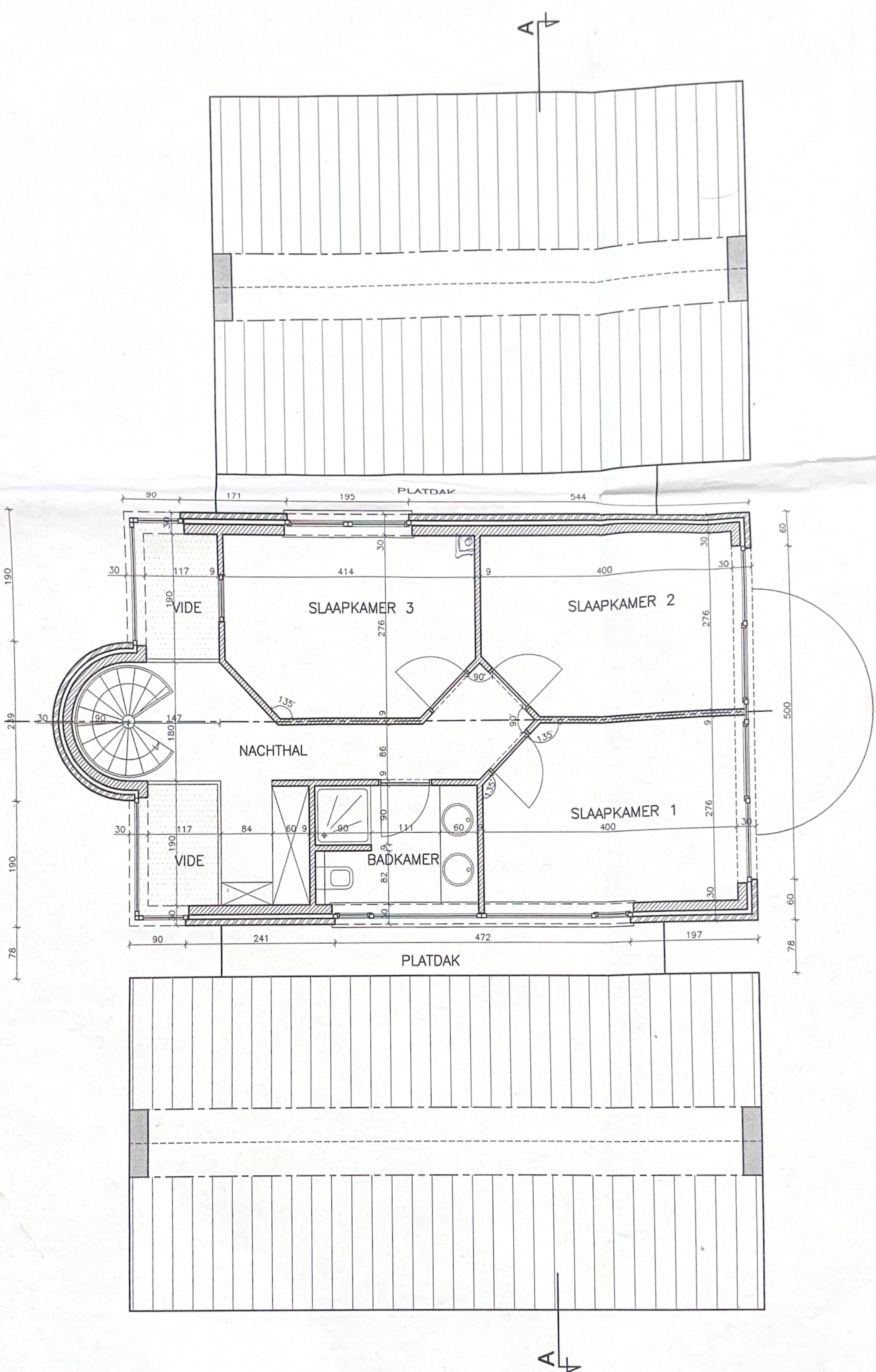
PLAN VERDIEPING
